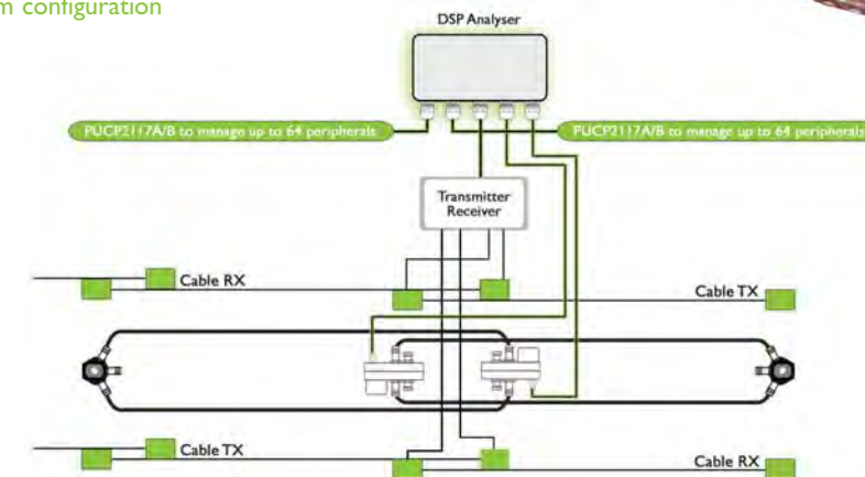
System configuration
