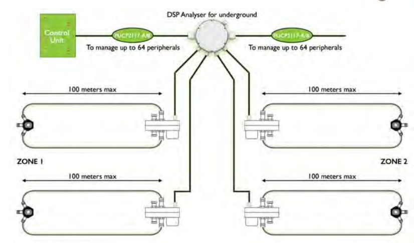
System configuration
